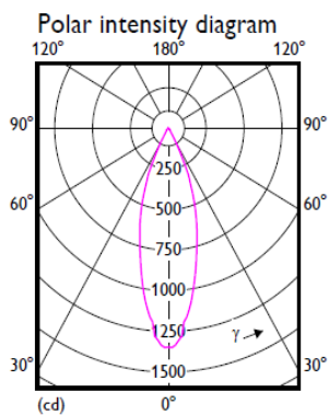
BGP150 LED G 8W 35D 1 x LED 1 x 500 lm
