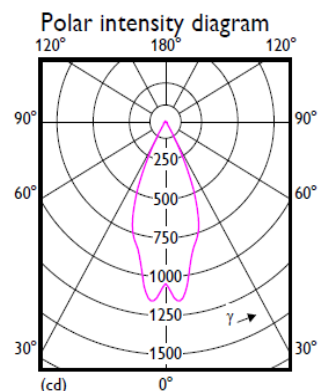
BGP150 LED580 NW 8W 45D 1 x LED 1 x 580 lm
