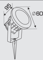
RC 04 LED 9W
