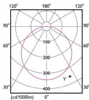
Downlight DN020 G3 CW 10,5W D150 GM
