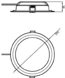
DN020 GM RR 900lm 6500K TBDW 6" WH ND
