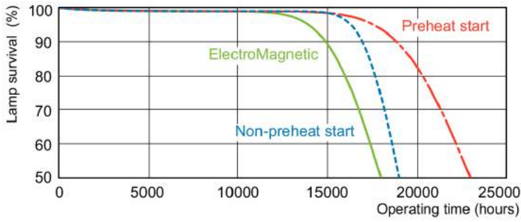
LDLE_TL-D9Hm_0002-Life expectancy diagram
