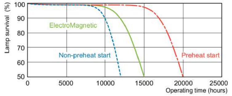
LDLE_TL-D9Hm_0001-Life expectancy diagram
