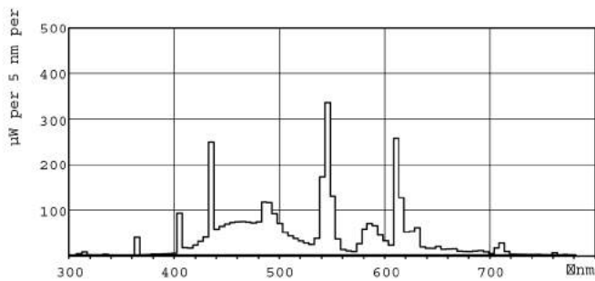
LDPB_TL-D9HLM_965-Spectral power distribution B/W
