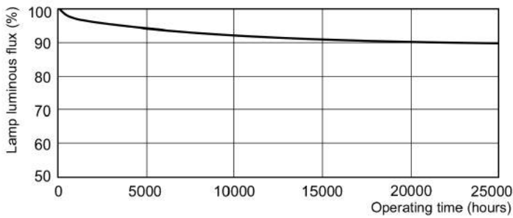
LDLM_TL-D9Hm_0001-Lumen maintenance diagram
