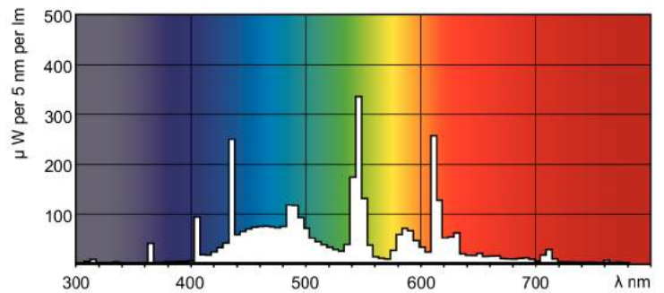
LDPO_TL-D9HLM_965-Spectral power distribution Colour
