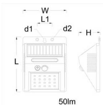
BWS010 LED50/765
