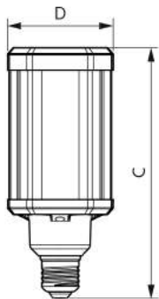
TrueForce LED HPL ND 28-21W E27 830
