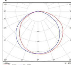
Light Distribution
