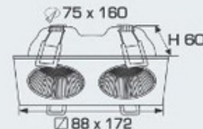
AFC 768/2 LED 12W 968.000
