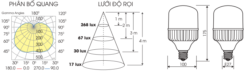
TR100ND2/30W
