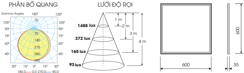
P06.UGR19 600x600/50W
