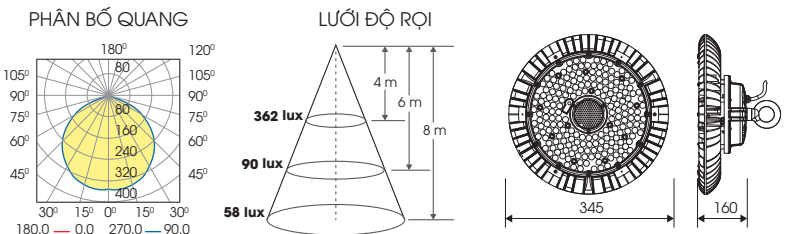
HB03 390/200W
