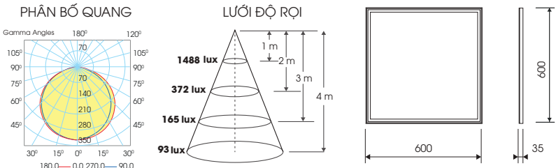
P06.UGR19.T 600x600/50W
