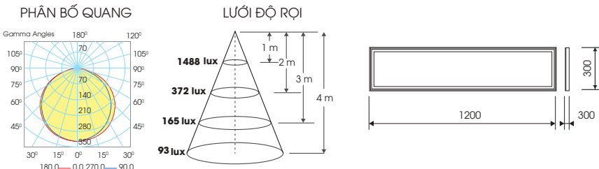
P06.UGR19 300x1200/50W
