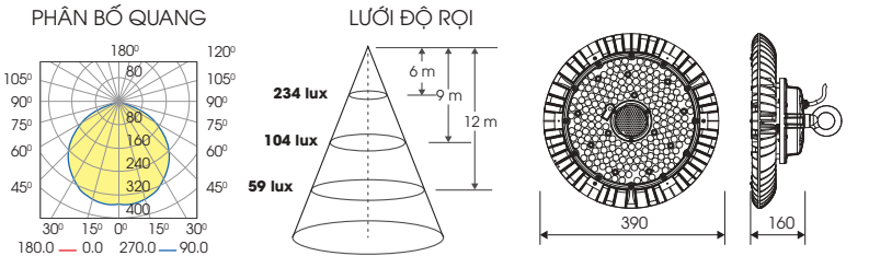
HB03 390/250W
