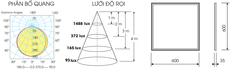
P06.UGR19.V 600x600/50W
