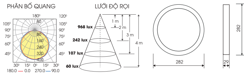
LN09 300/30W
