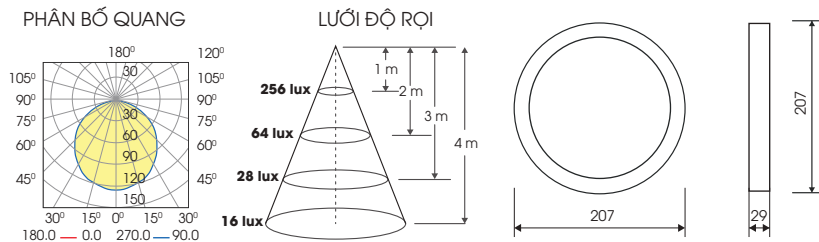
LN09 220/22W
