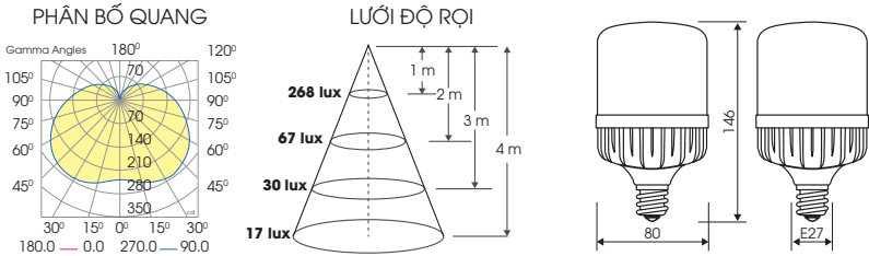
TR80ND2/20W
