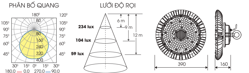
HB03 390/200W
