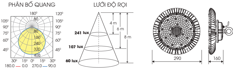
HB03 350/120W
