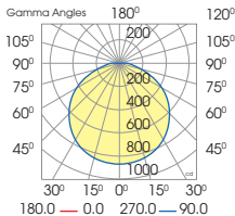
LN16 540x540/40W
